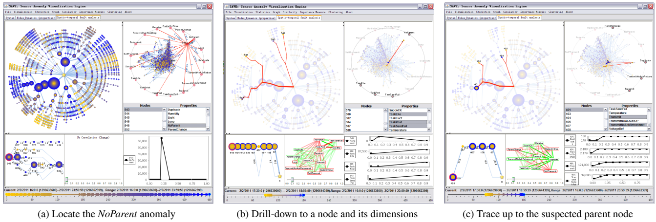
Figure 9: Link failure diagnosis: the user starts by locating the NoParent anomaly in node 543 (Figure (a)), drills down to the node and abnormal time range to show the topology, dimension and correlations (Figure (b)), traces up to the suspected ancestral node 401 for in-situ analysis (Figure (c)), finally validates node 457 to be normal and concludes with the link failure between node 401 and 457 (Figure 11).
